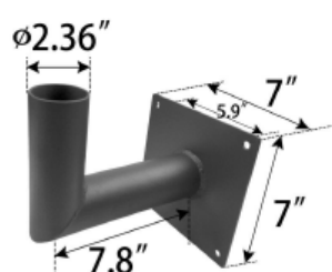
LOT-MO-PW-19 90 Degree Pole Adapter
