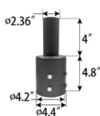
LOT-MO-PW-8 4" Round Pole Adapter
