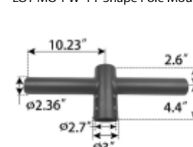
LOT-MO-PW-4 T-Shape Pole Mount
