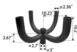
LOT-MO-PW-13 4-Arm Pole Adapter
