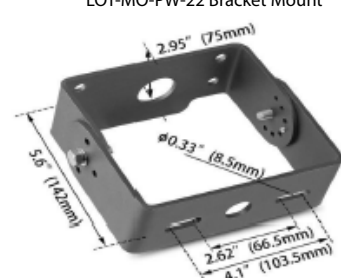
LOT-MO-PW-22 Bracket Mount
