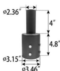
LOT-MO-PW-7 3" Round Adapter
