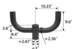
LOT-MO-PW-12 U-Shape Pole Adapter
