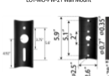
LOT-MO-PW-21 Wall Mount
