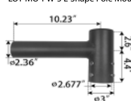
LOT-MO-PW-5 L-Shape Pole Mount
