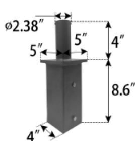
LOT-MO-PW-2 5" Square Pole Adapter
