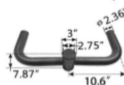
LOT-MO-PW-14 Bull Horn Adapter
