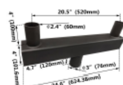
LOT-MO-PW-15 2-Head Pole Adapter
