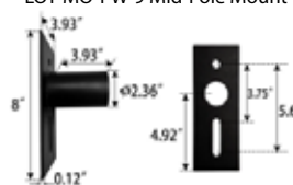
LOT-MO-PW-9 Mid-Pole Mount
