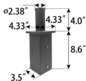
LOT-MO-PW-1 4" Square Adapter
