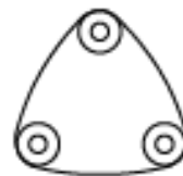
Base Footprint Triangular base pattern requiring three (3) 3/4" anchor bolts
