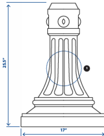
1. Access Door Height 9.5" Width 11"
